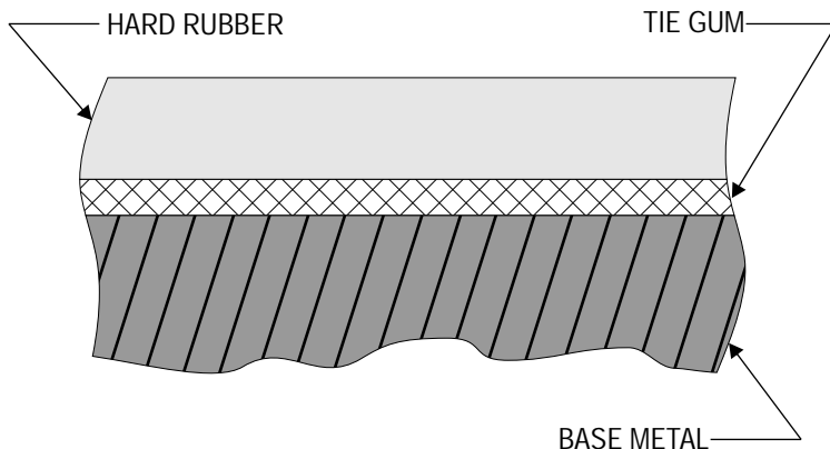
Figure 3: Cross Section
