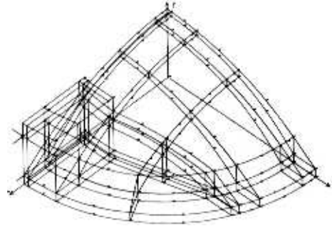
Figure 1: Domed Disc Finite Element Model (quarter section)
