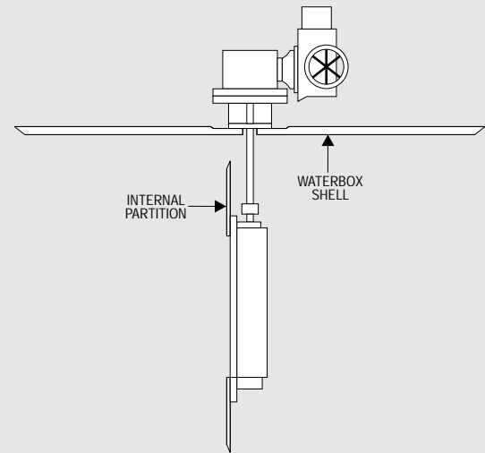
Figure 5: Condenser Partition Valve – Typical Installation
