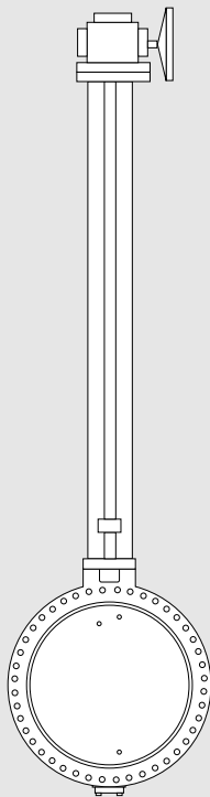
EXTENSION BONNET AND SHAFT
