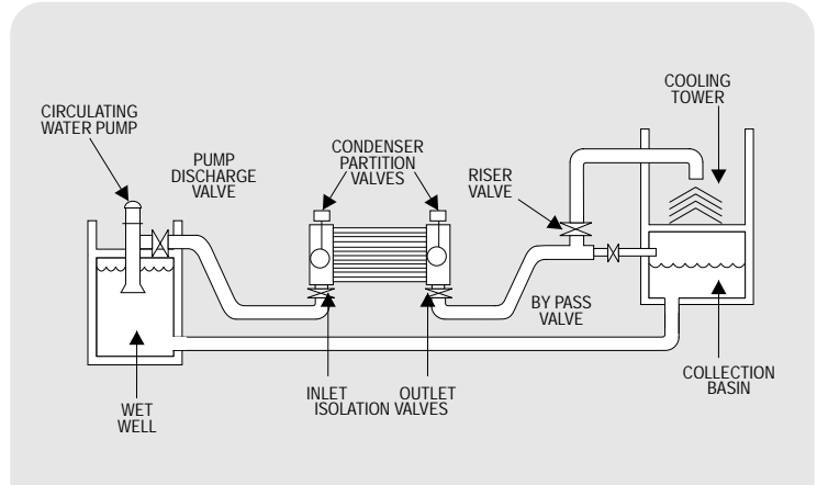
Figure 4: Typical Circulating Water System
